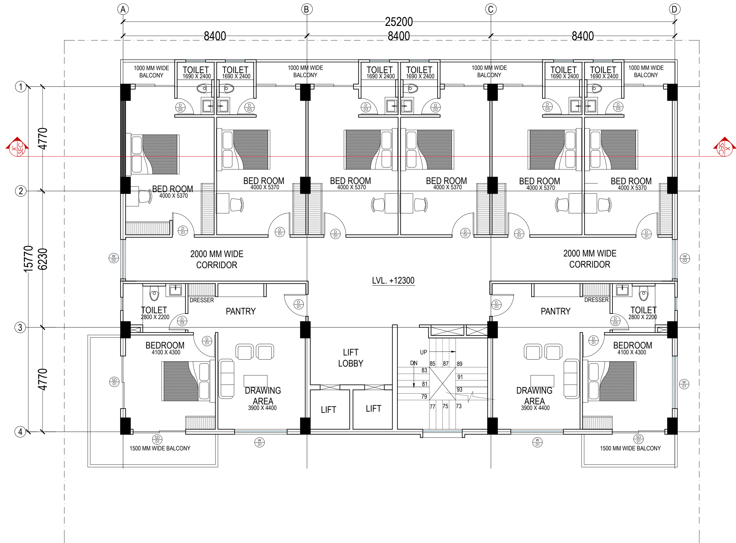
FOURTH FLOOR AREA 406 SQ.MT.
