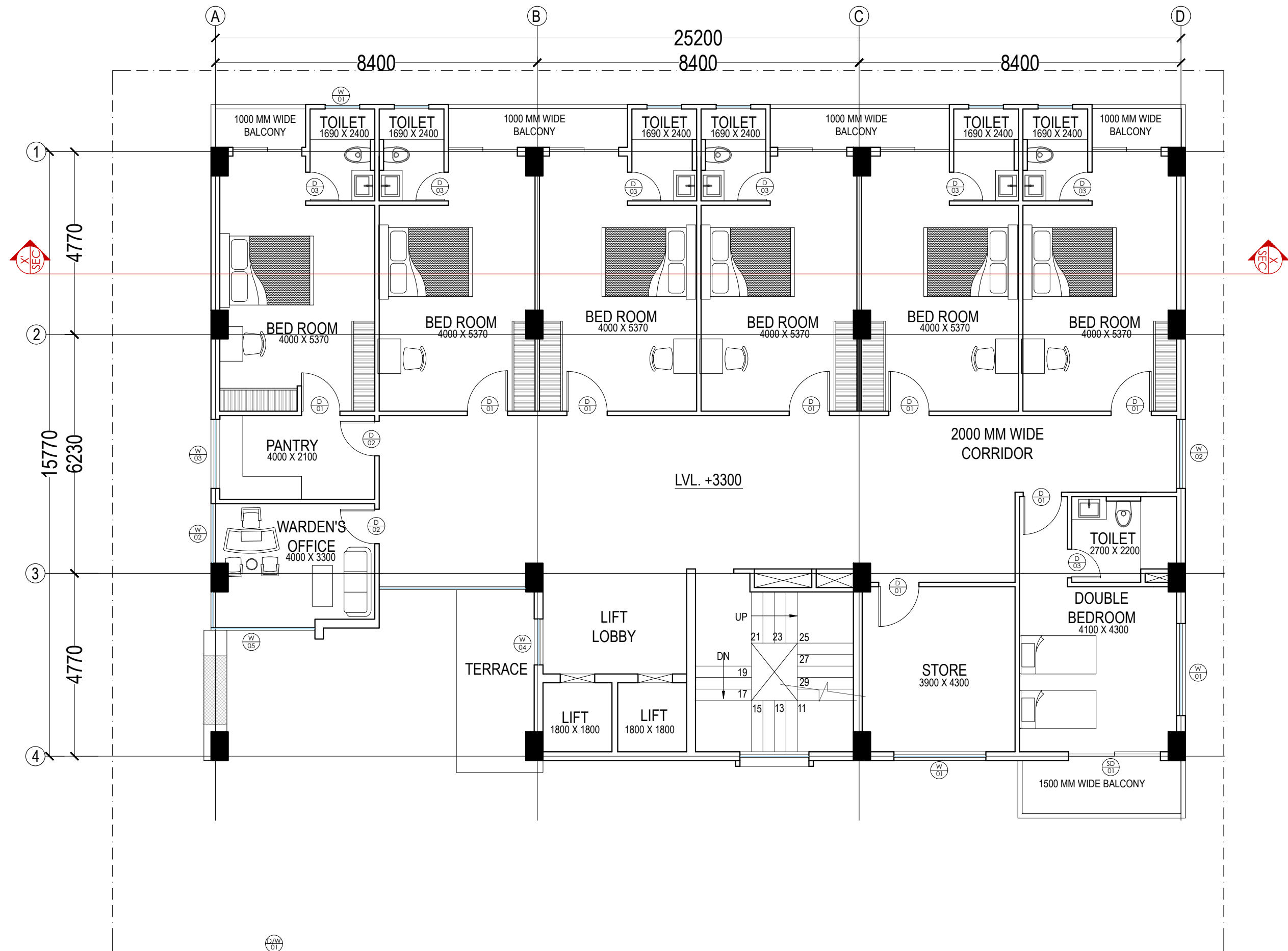
FIRST FLOOR AREA 386 SQ.MT.
