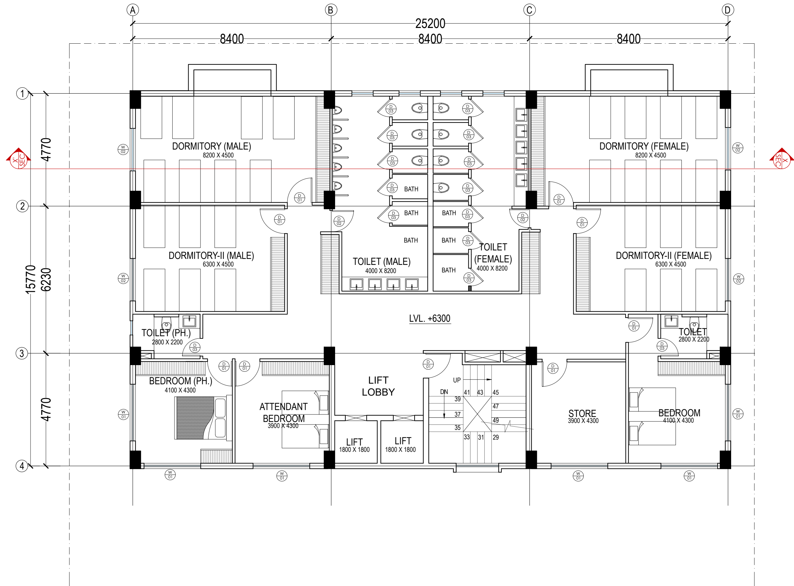
SECOND FLOOR AREA 406 SQ.MT.
