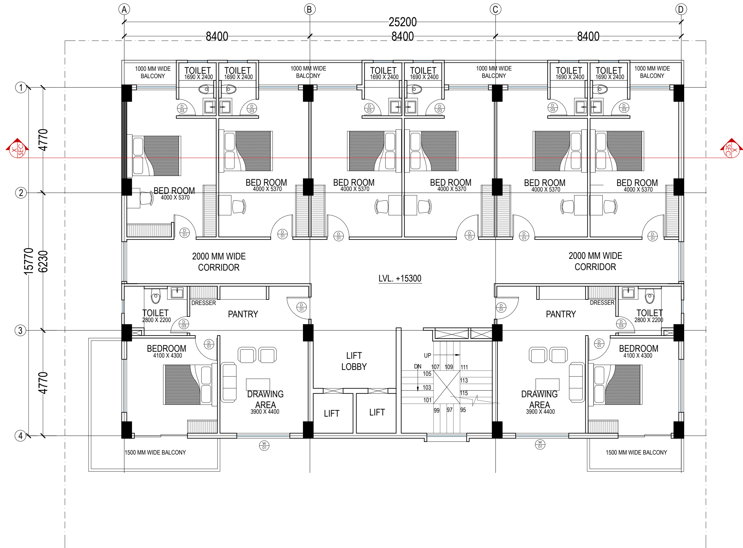
FIFTH FLOOR AREA 406 SQ.MT.
