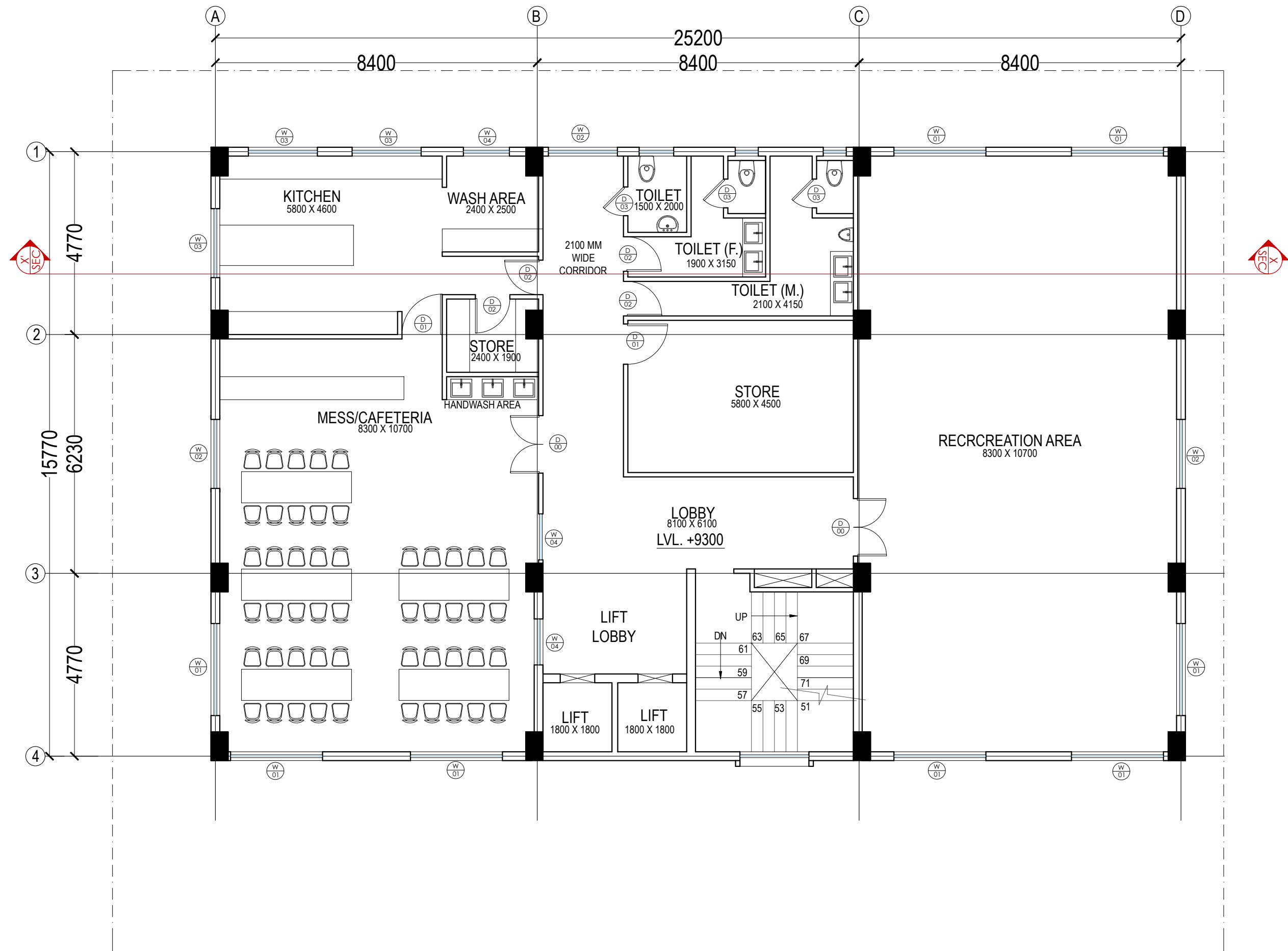
THIRD FLOOR AREA 406 SQ.MT.
